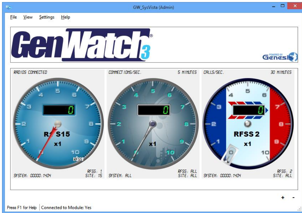
Figure 1.8 – Multi-View Window
