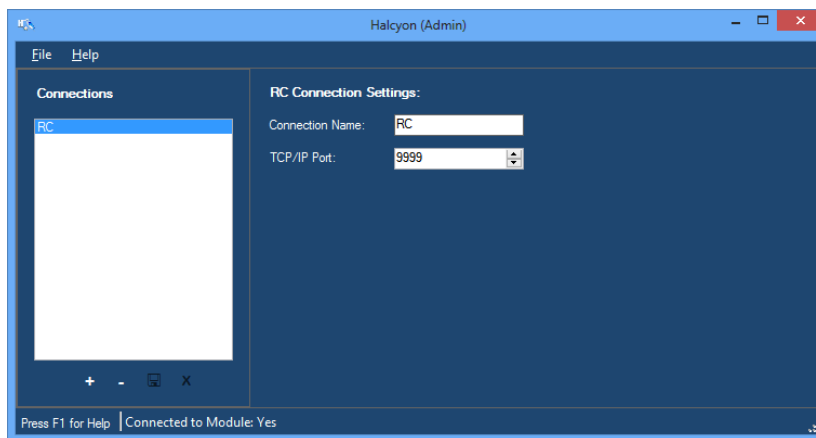
Figure 1.1 – Halcyon GUI
