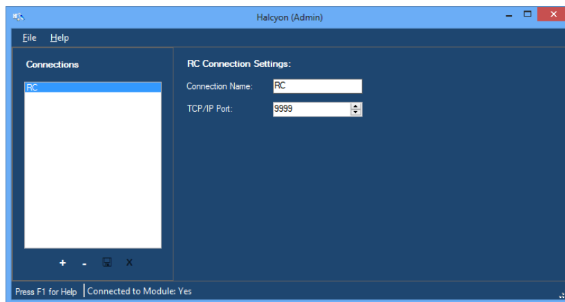
Figure 1.1 – Halcyon GUI
