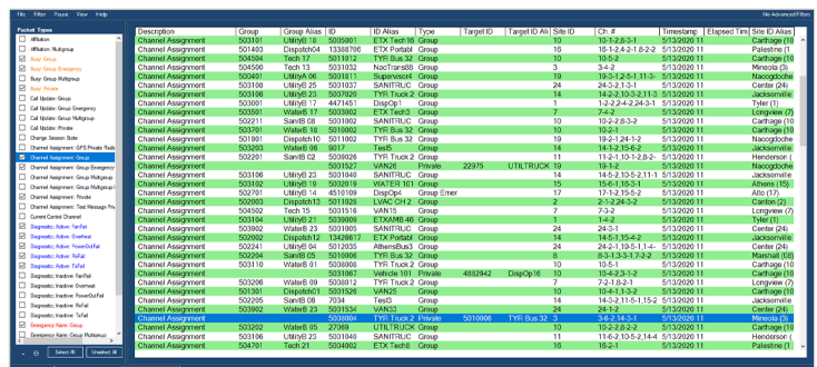
Figure 8: Activity Module
