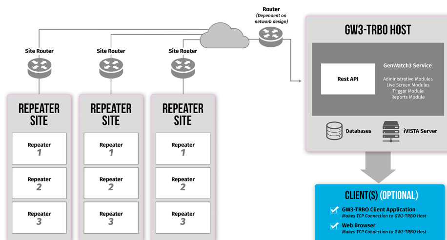
Figure 2: GW3-TRBO Connects to Capacity Plus Multi-Site
