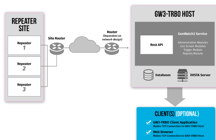
Figure 1: GW3-TRBO Connects to Capacity Plus Single Site
