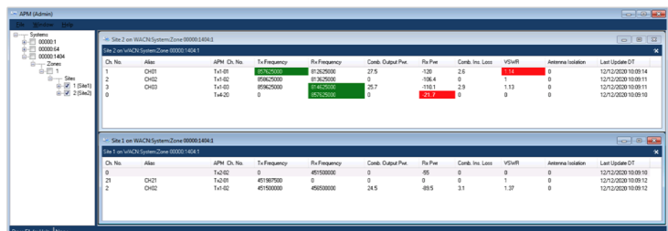
Figure 11: APM Module
