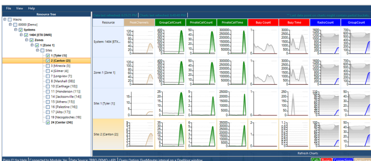
Figure 10: KPI Module
